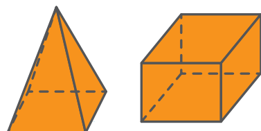
Irregular Polyhedrons
