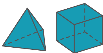
Regular Polyhedrons
