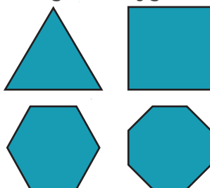
Regular Polygons
