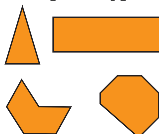
Irregular Polygons
